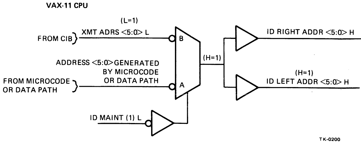
Figure 1-3 ID Bus Control Logic, Block Diagram
