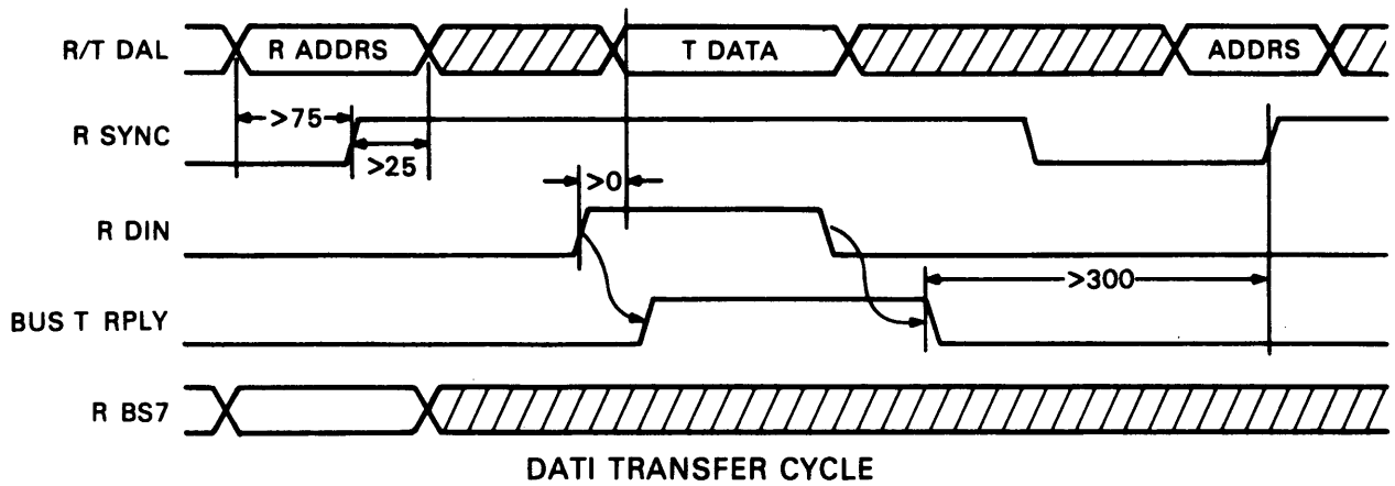
Figure 3-10 DATI Transfer Timing on the Q Bus
