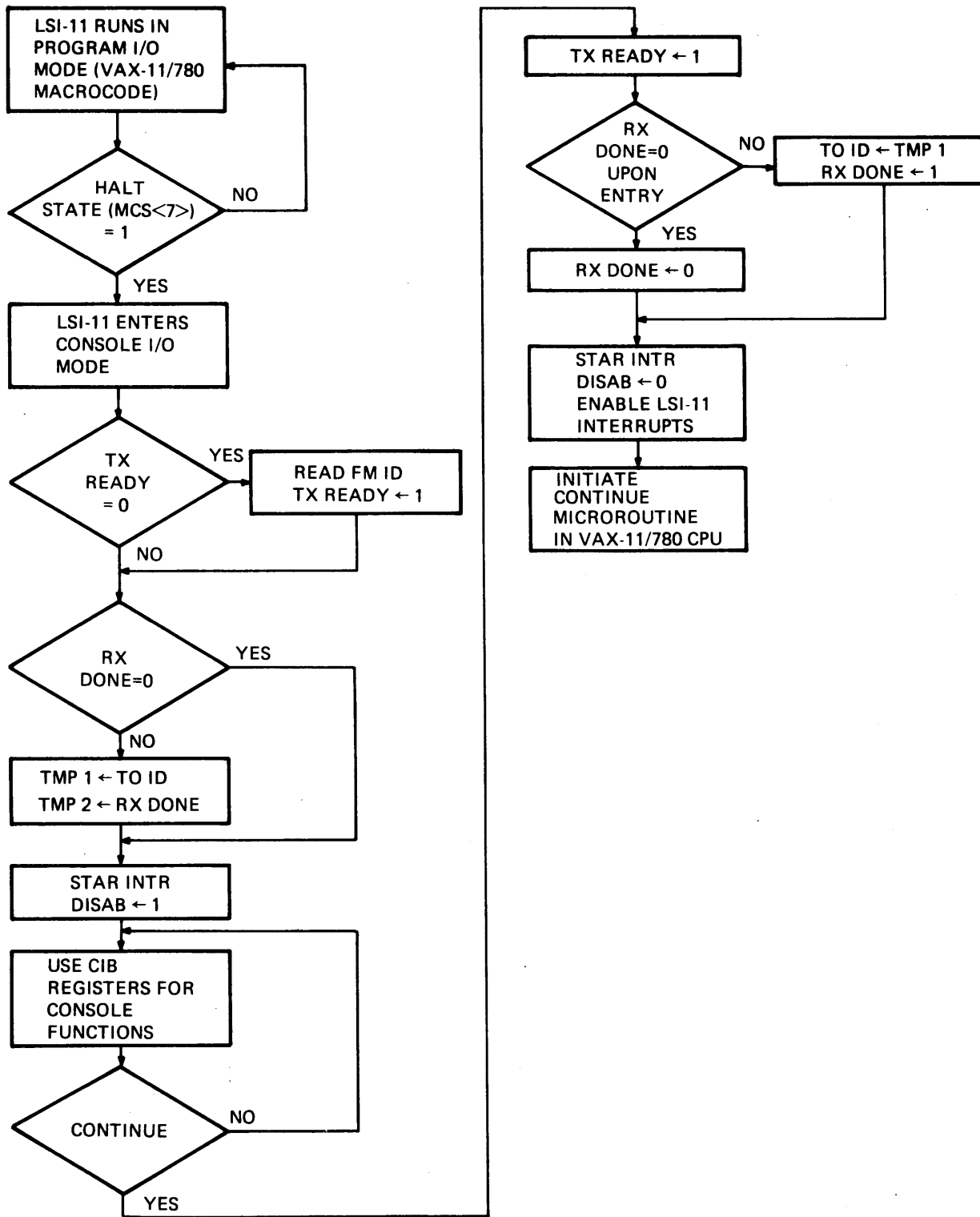
Figure 2-10 LSI-11 Response to a VAX-11/780 CPU Halt
