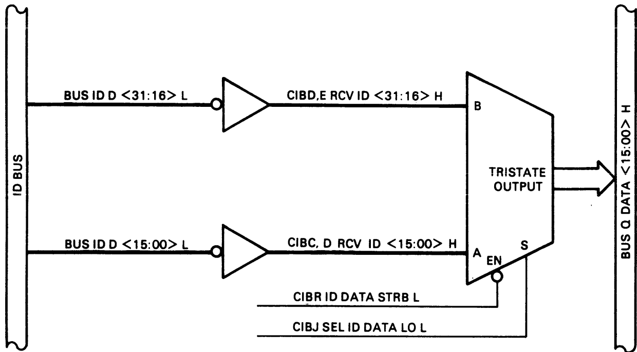
Figure 3-22 ID DATA HI and ID DATA LO Register Logic
