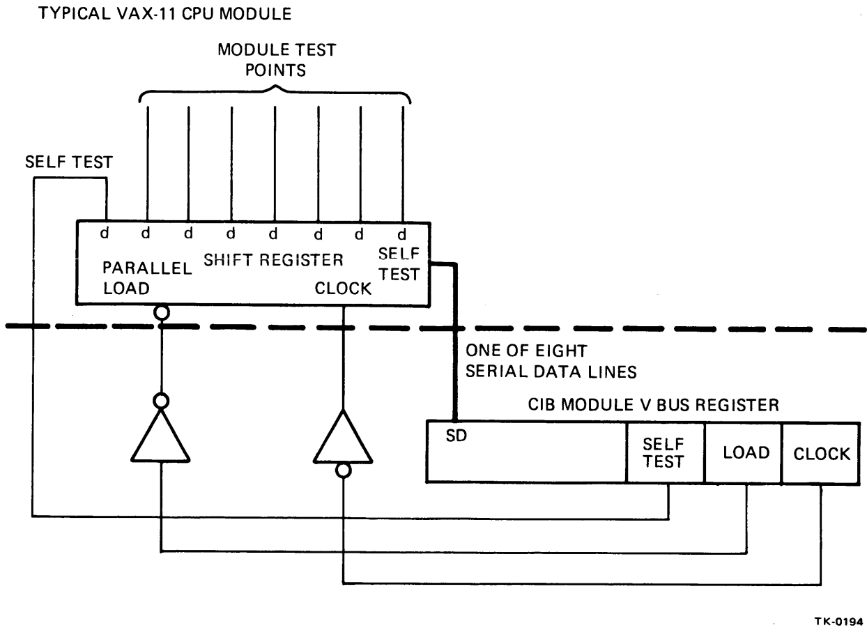
Figure 1-4 V Bus Block Diagram
