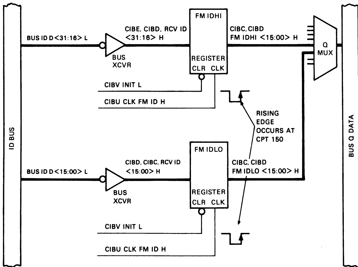
Figure 3-16 FM ID Register Logic
