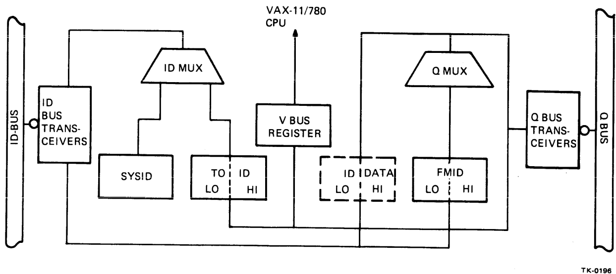
Figure 2-2 CIB Data Paths, Simplified Block Diagram
