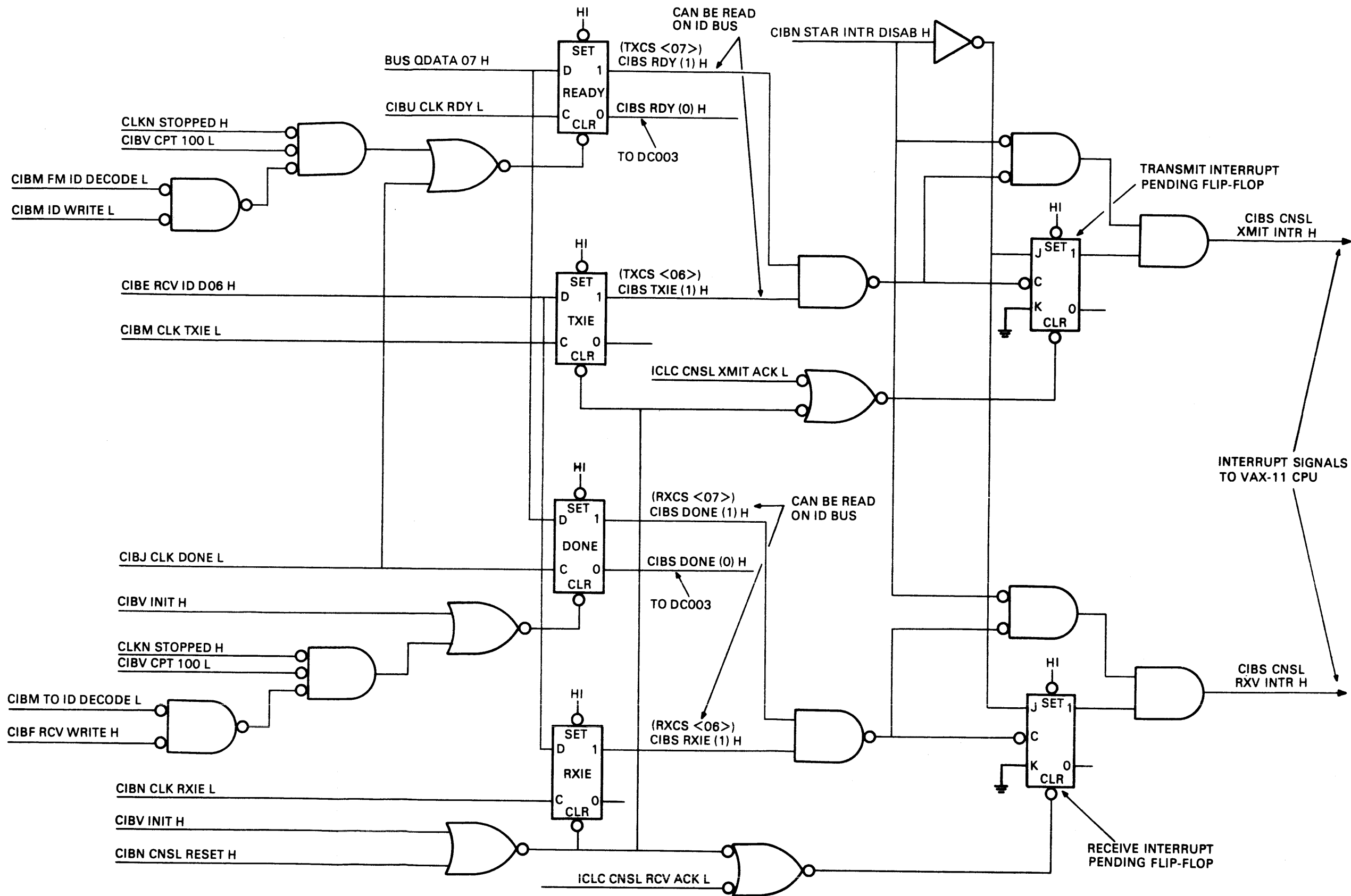
Figure 3-23 VAX-11/780 CPU Interrupt Logic
