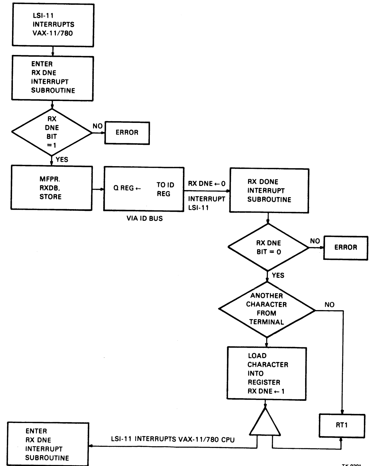
Figure 2-8 LSI-11 Sends a Character to the VAX-11/780 CPU, Flowchart
