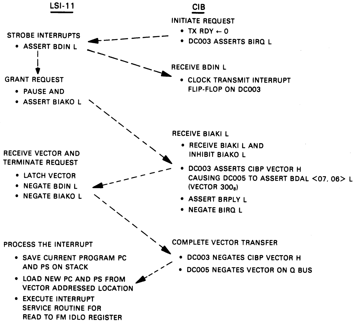
Figure 3-28 Interrupt Dialogue on the Q Bus
