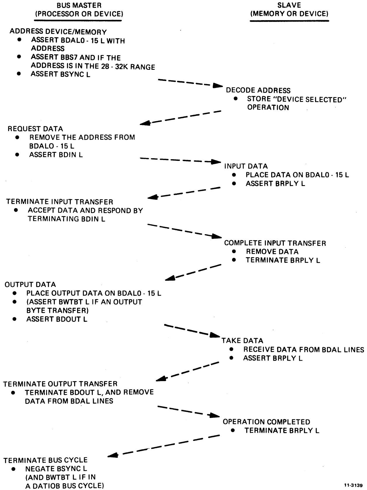
Figure A-2 DATIO or DATIOB Bus Cycle
