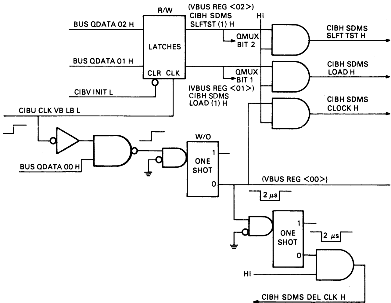
Figure 3-20 V Bus Register Logic
