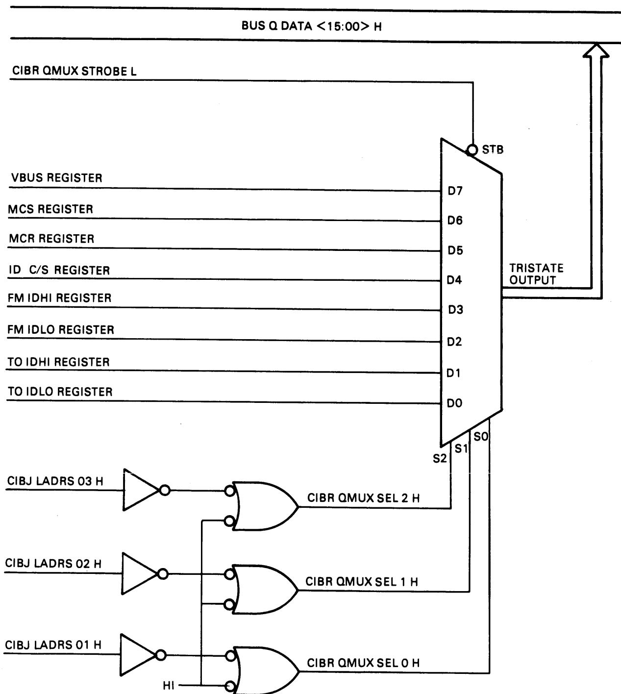
Figure 3-4 QMUX Logic
