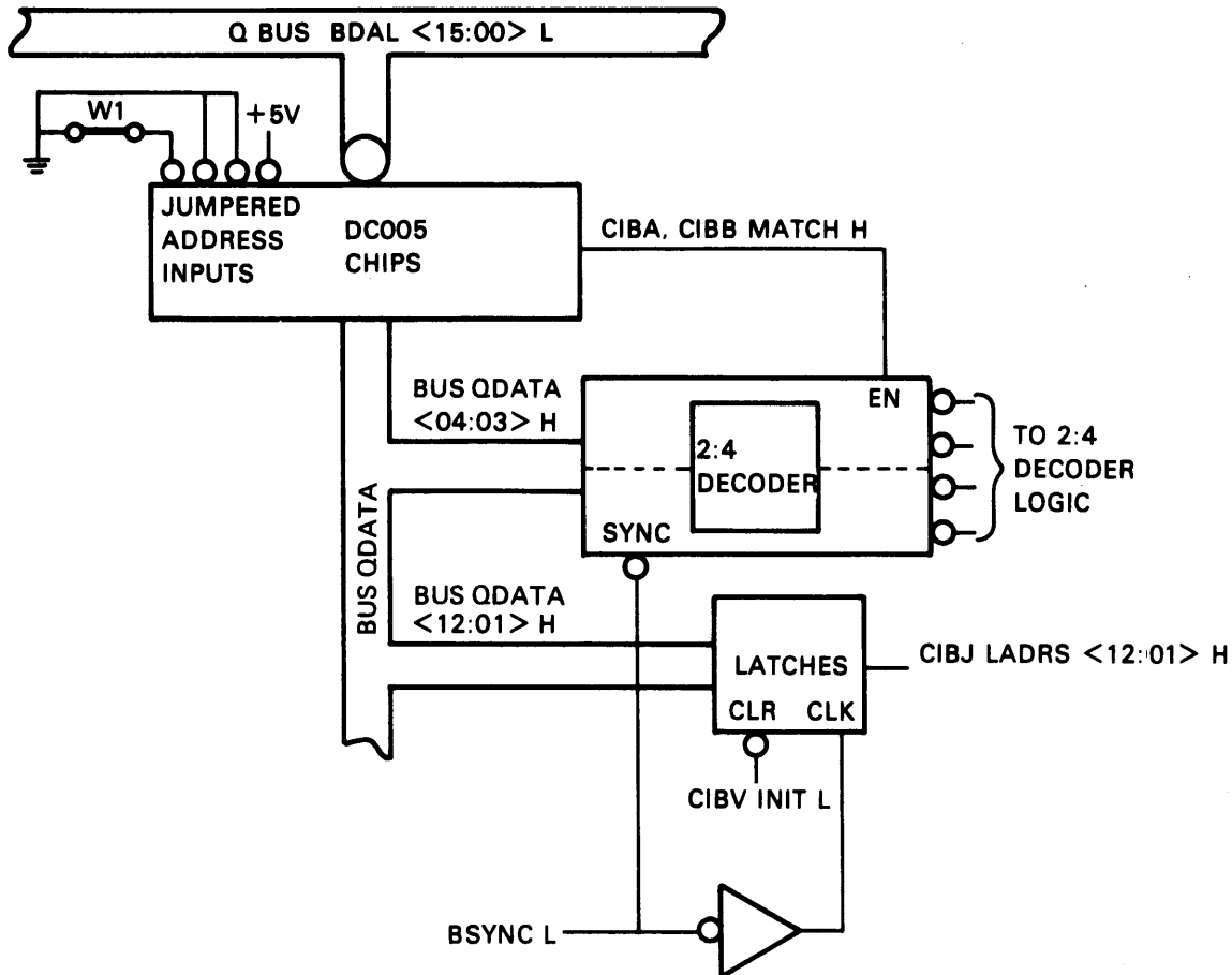
Figure 3-3 Q Bus Address Decoder Logic Interface Chips
