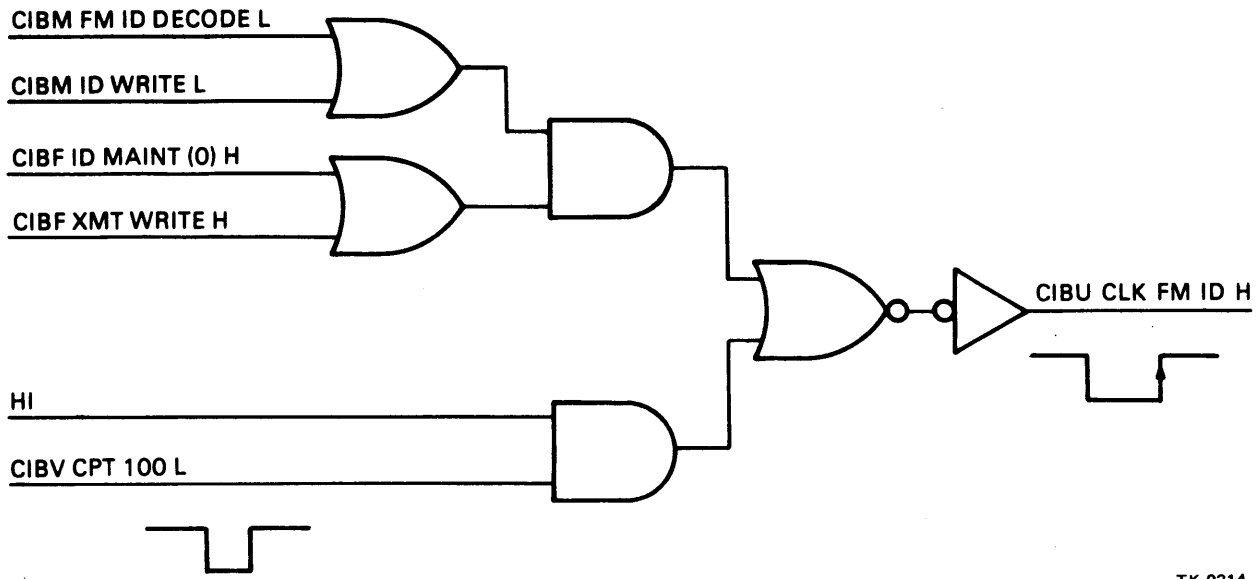
Figure 3-15 Development of CIBU CLK FM ID H
