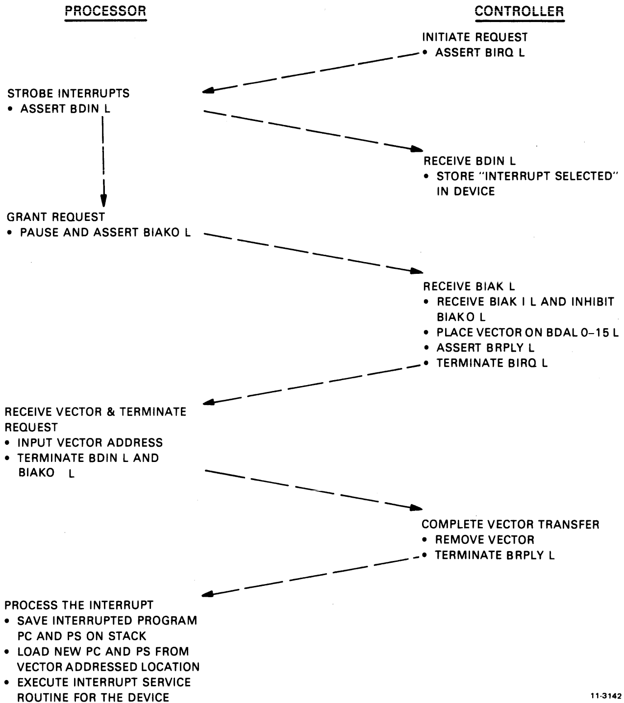
Figure A-4 Interrupt Request/Acknowledge Sequence
