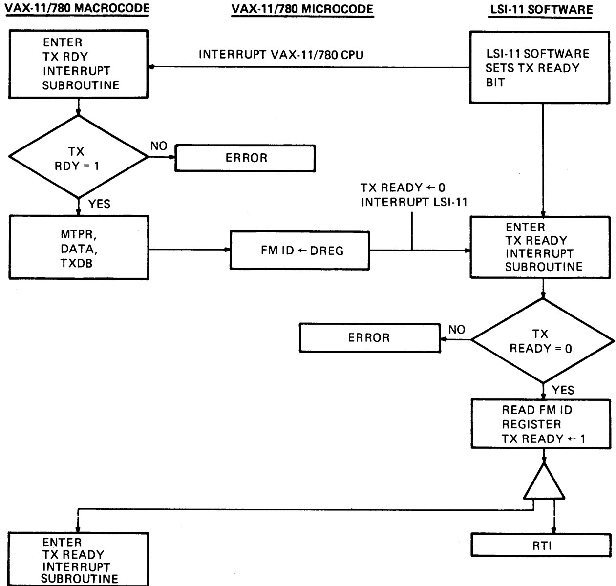
Figure 2-9 VAX-11/780 Sends a Character to the LSI-11, Flowchart
