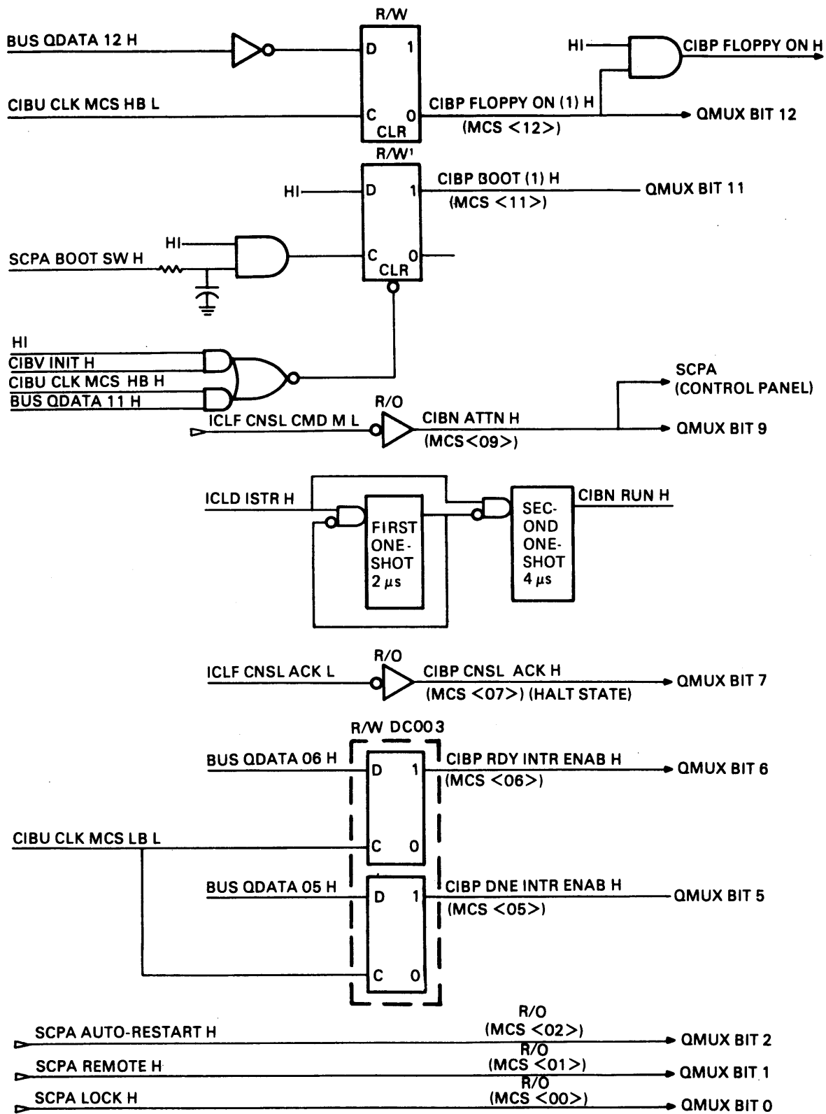
Figure 3-19 MCS Register Logic
