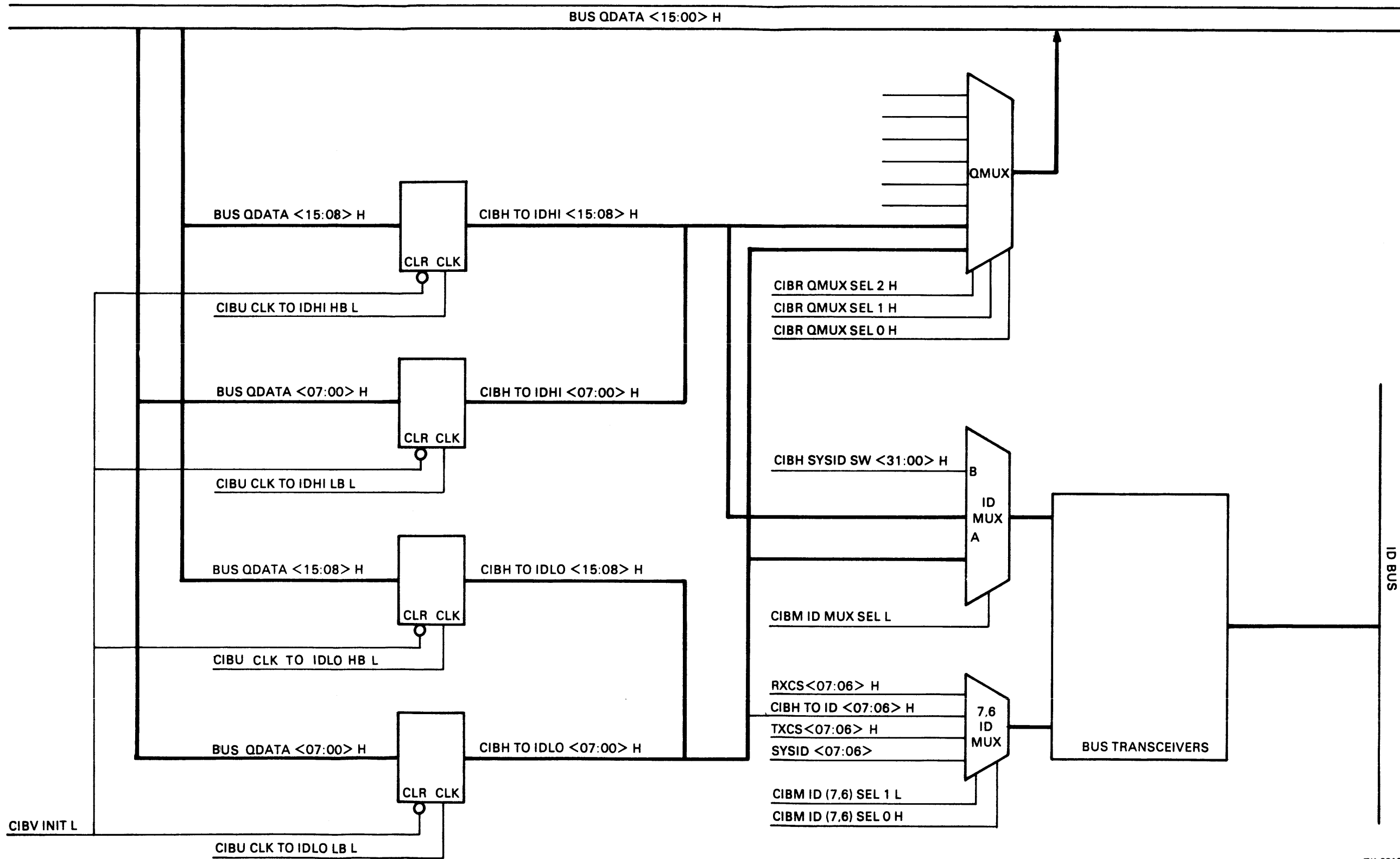
Figure 3-14 TO ID Register Logic
